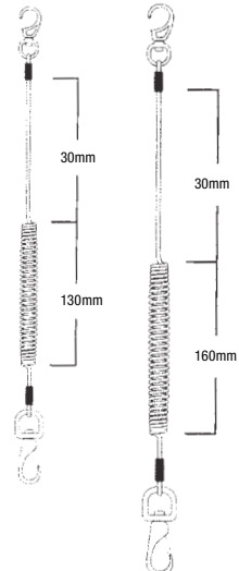
5kg Load weight Part No. 301907 10kg Load weight Part No. 301908
